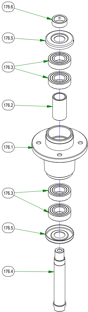
037-4000-00 SPINDLE ASSEMBLY
