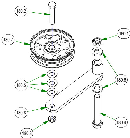
039-0031-19 REAR IDLER PULLEY
