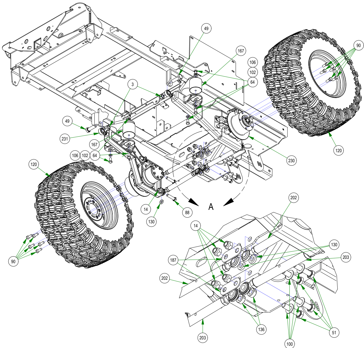
DETAIL A
